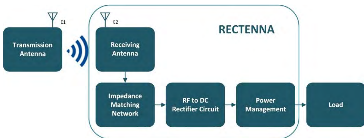
Figure 1. Block diagram of a typical RF harvesting system.
