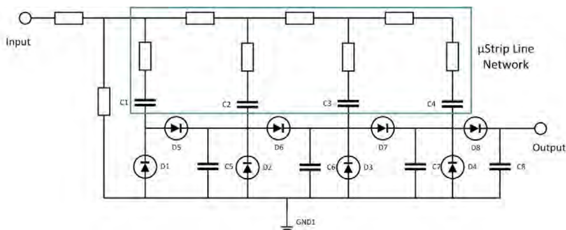
Figure 6. L-network in combination with the microstrip line network is equivalent to the T- Impedance Matching Network (IMN).
