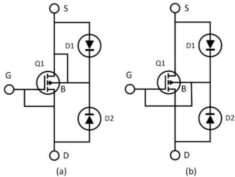
Figure 11. Diode connected transistors: (a) BTMOS (b) DTMOS.
