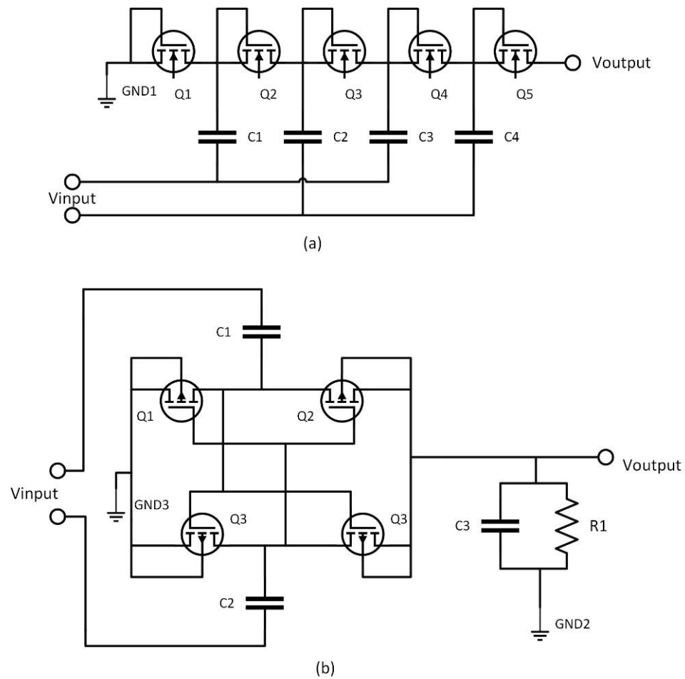
Figure 10. CMOS rectifier topologies: (a) Dickson Charge Pump (b) Differential Voltage Multiplier.
