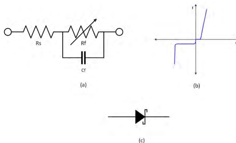
Figure 7. The characteristics of a diode (a) electronic equivalent circuit (b) I-V characteristic of Schottky diode (c) symbol of Schottky diode.
