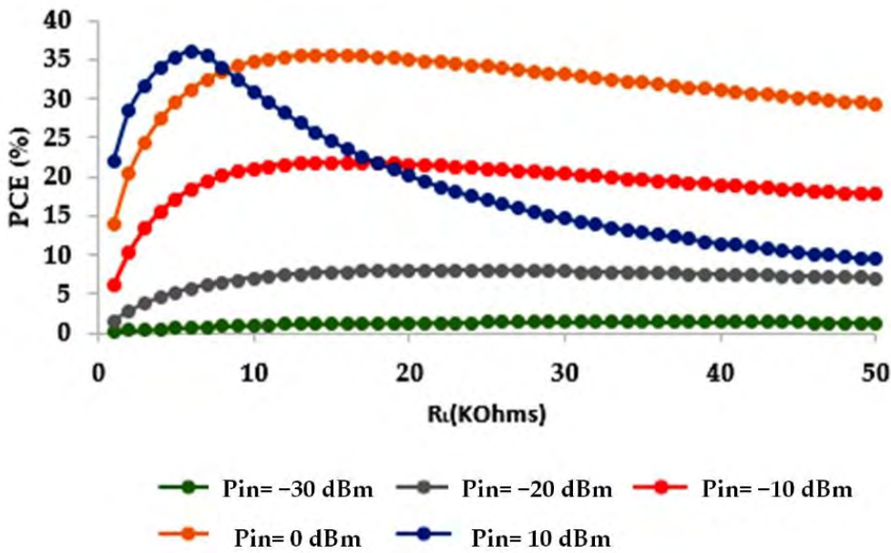
Figure 13. The change of PCE depends on different output loads.
