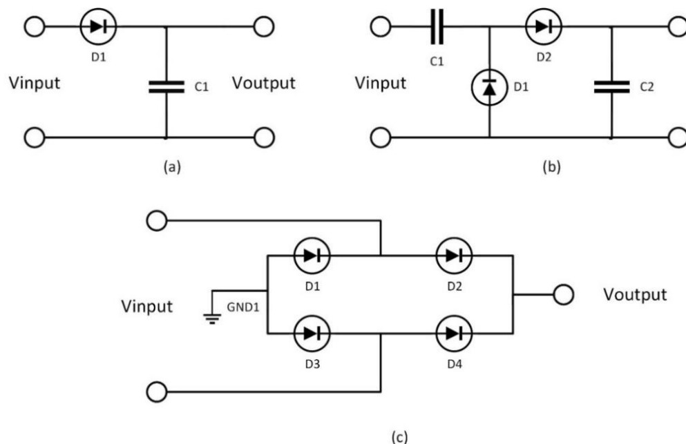
Figure 8. Types of rectifier configurations: (a) half-wave rectifier (b) full-wave rectifier (c) bridge rectifier [11].
