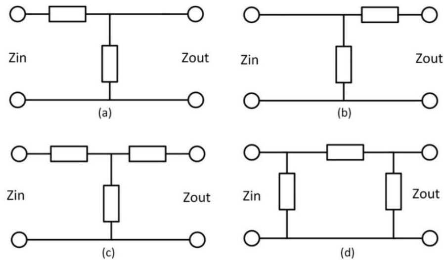
Figure 4. Different types of impedance matching networks with distributed elements: (a) L-network, (b) Reversed L-network, (c) T-network, (d) \pi -network [1].
