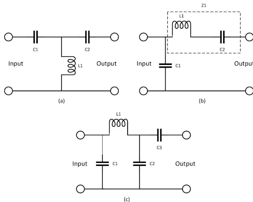
Figure 5. Different types of impedance matching networks with lumped elements: (a) T-Network (b) L-Network (c) \pi -Network.
