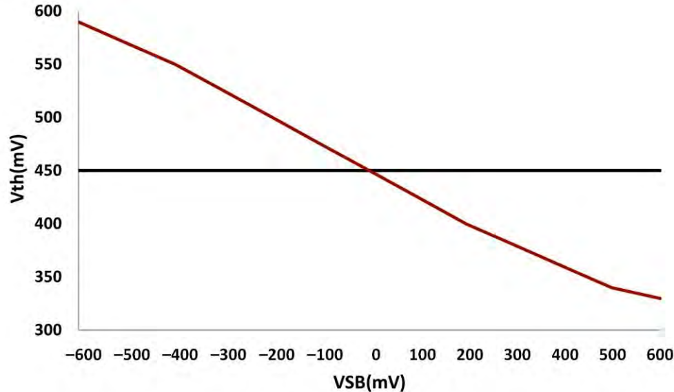
Figure 12. V_{T}-V_{SB} (The red color refers to DTMOS and the dark blue to BTMOS).
