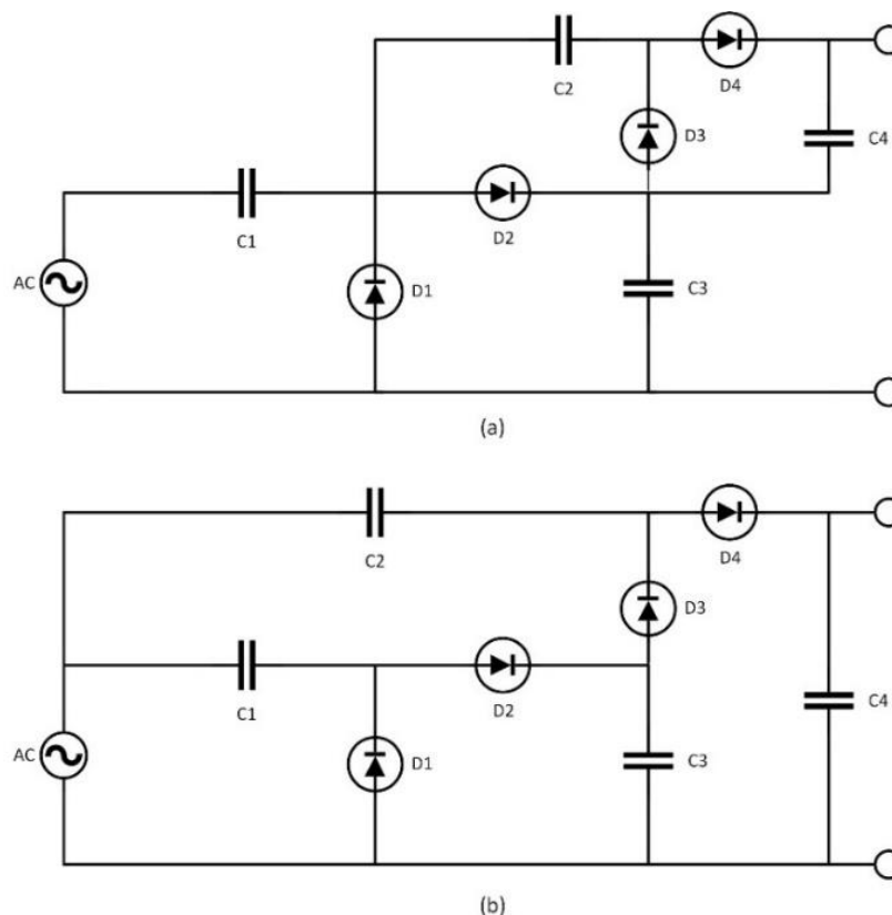
Figure 9. Topologies of voltage multipliers: (a) Villard Topology (b) Dickson Topology.
